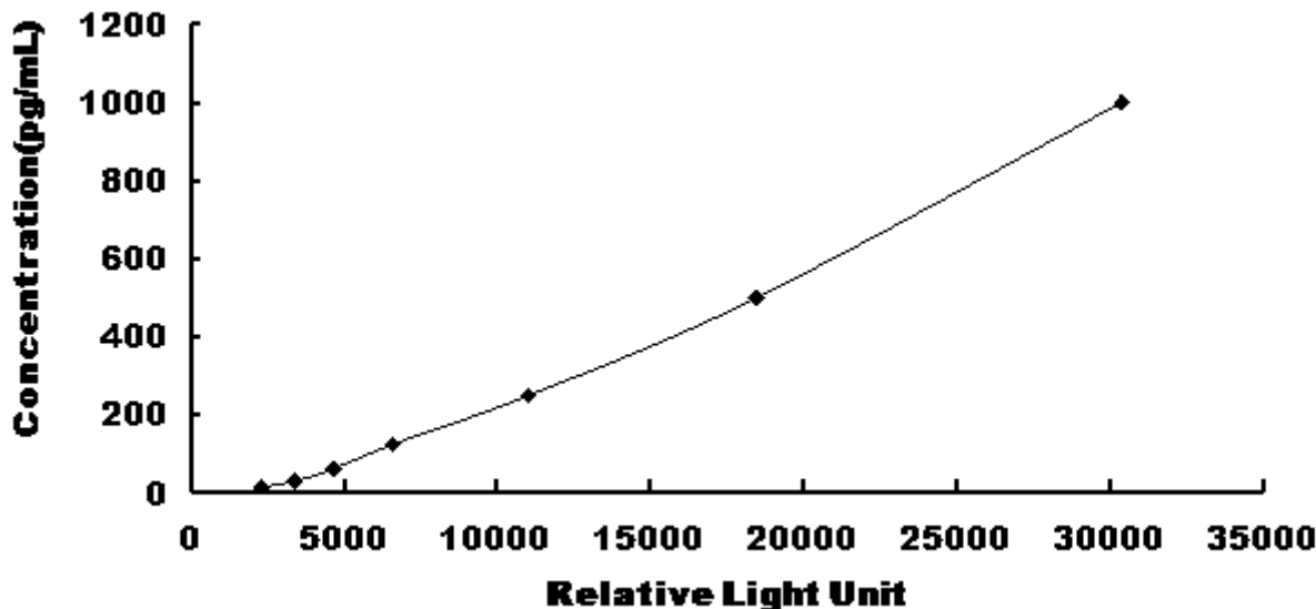
Typical Standard Curve for Bovine HGF CLIA.
