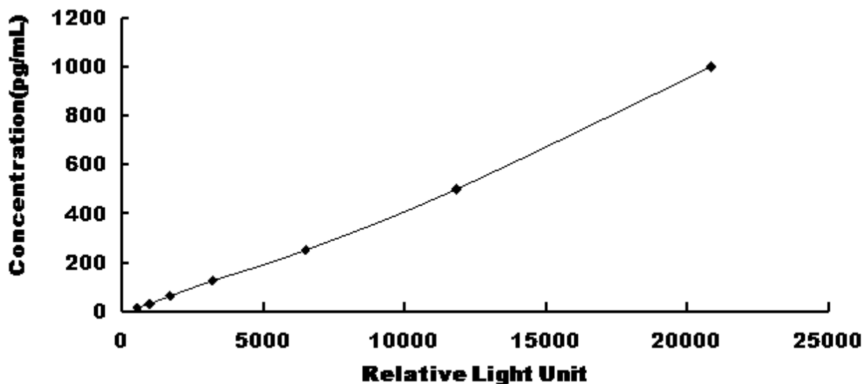
Typical Standard Curve for Human GCSF CLIA.
