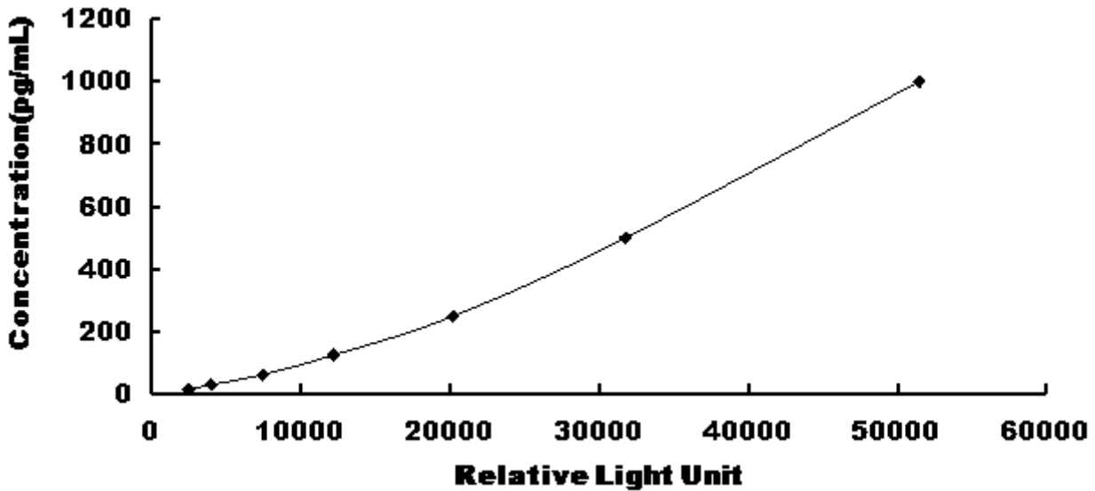
Typical Standard Curve for Human FGF1 CLIA.
