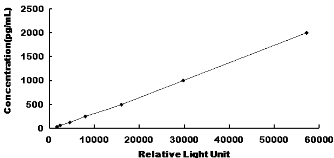
Typical Standard Curve for Canine BMP4 CLIA.
