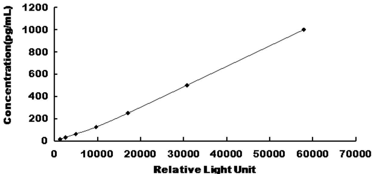
Typical Standard Curve for Mouse AREG CLIA.
