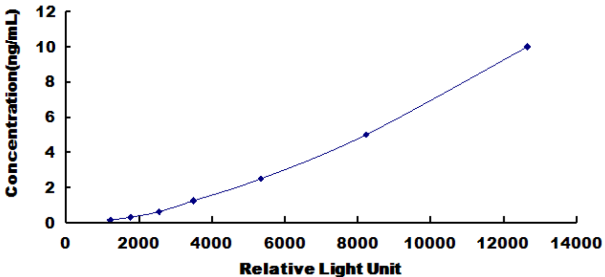
Typical Standard Curve for Rat EDRF1 CLIA.
