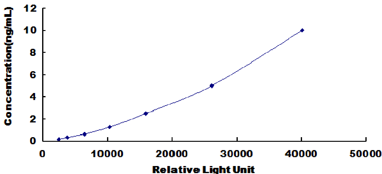
Typical Standard Curve for Human WNT1 CLIA.
