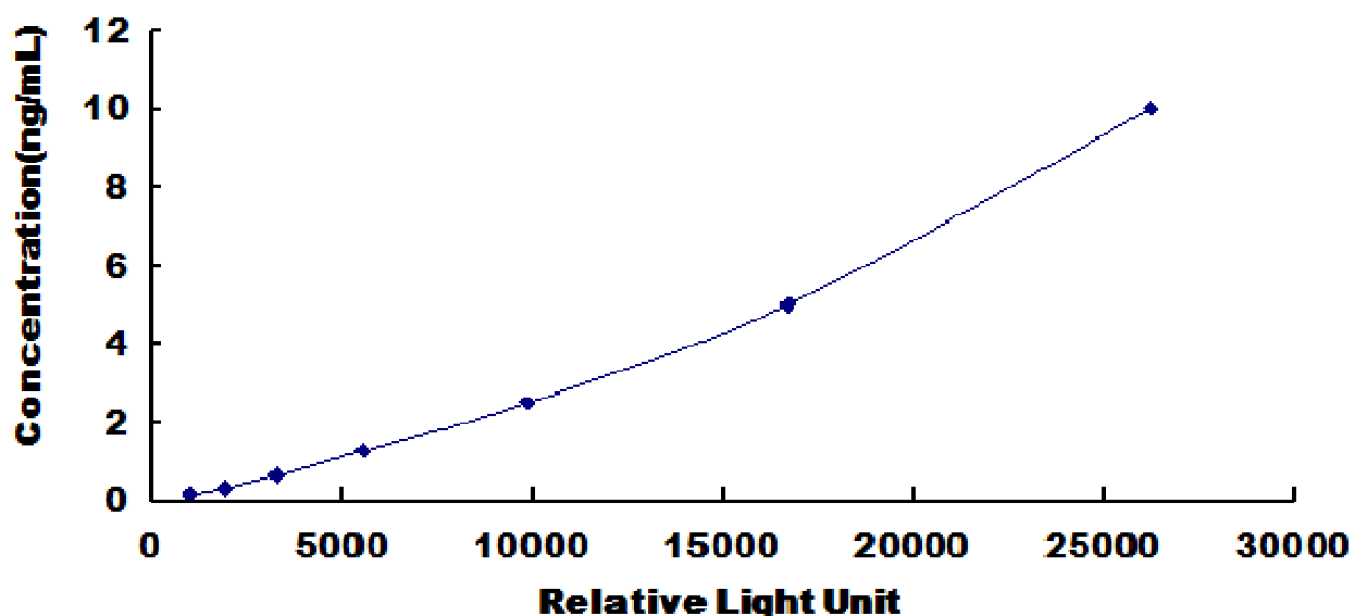
Typical Standard Curve for Human WNT3 CLIA.
