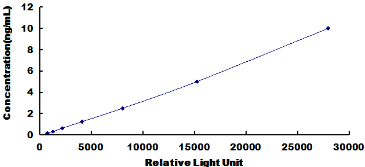
Typical Standard Curve for Mouse UCRP CLIA.
