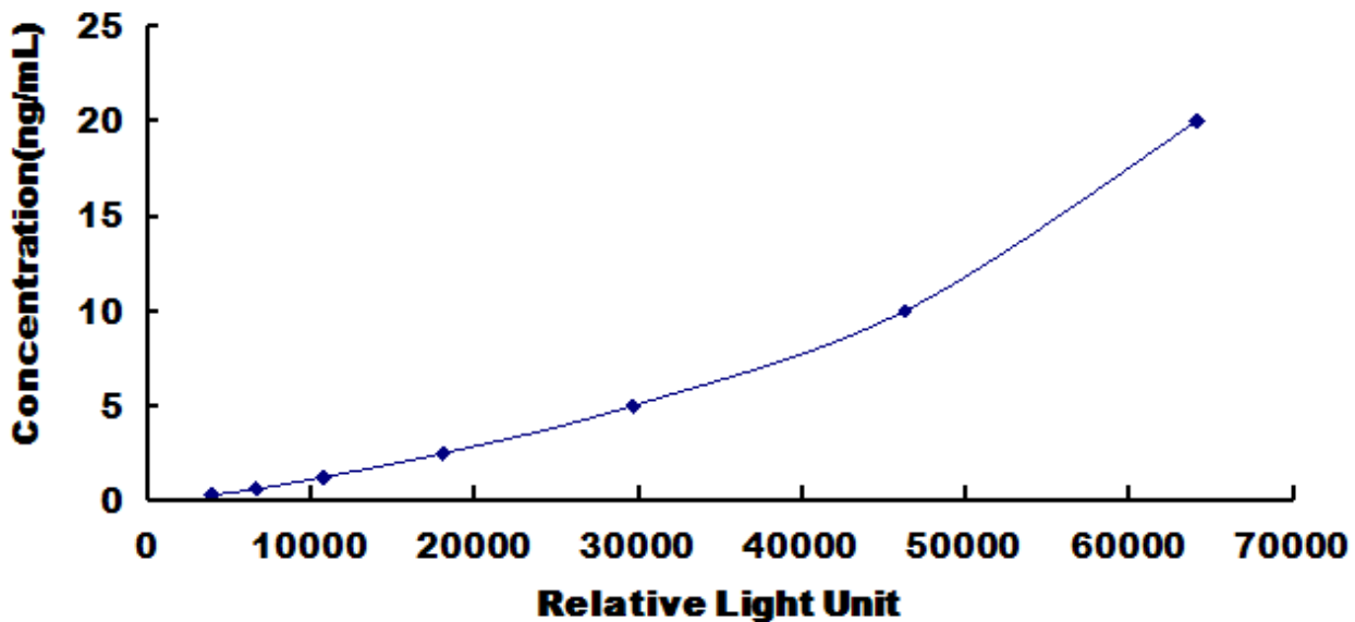
Typical Standard Curve for Human IGF2BP3 CLIA.
