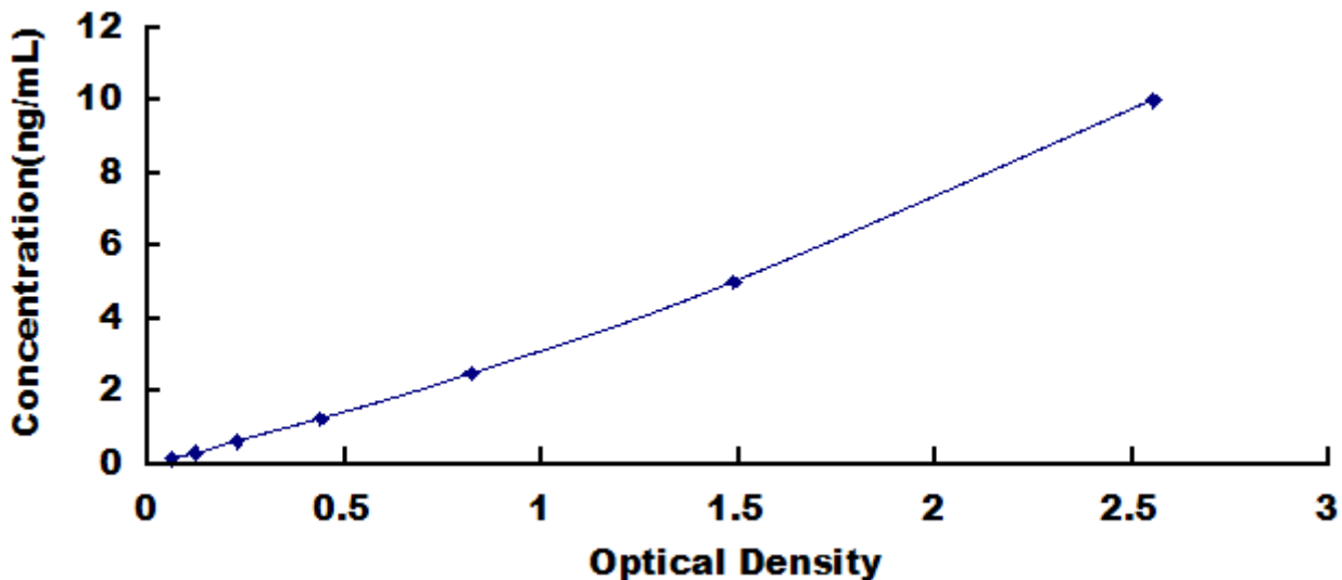
Typical Standard Curve for NUCB2, Human ELISA.
