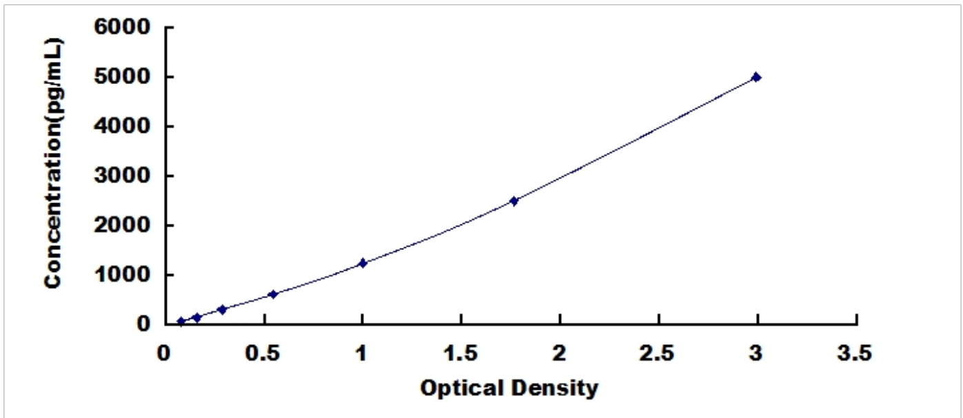
Typical Standard Curve for MIg, Bovine ELISA.
