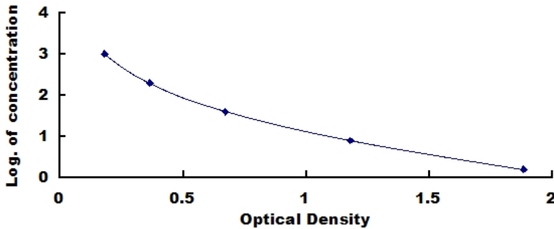
Typical Standard Curve for INHbA, Bovine ELISA.
